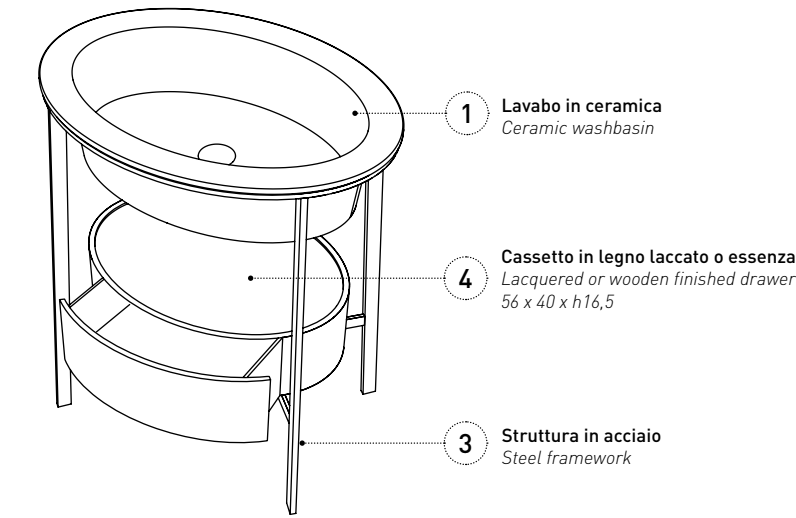
Catino Ovale 70 con cassetto Catino Ovale 70 with drawer 70 x 50 x h83
