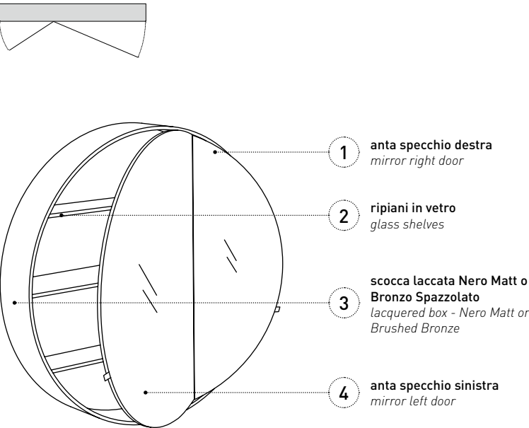
Specchio Round Box Round Box mirror Ø90 x 12 cm
