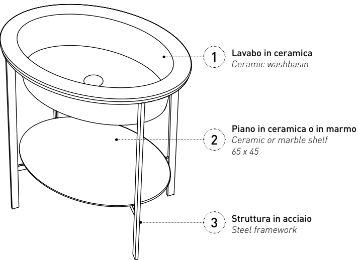
Catino Ovale 70 con piano Catino Ovale 70 with shelf 70 x 50 x h83
