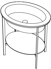
Catino 70 con piano Catino 70 with shelf 70 x 50 x h83
